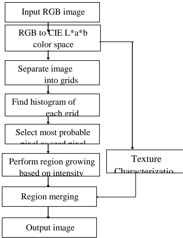
Figure 1. Block diagram of the proposed region growing algorithm
